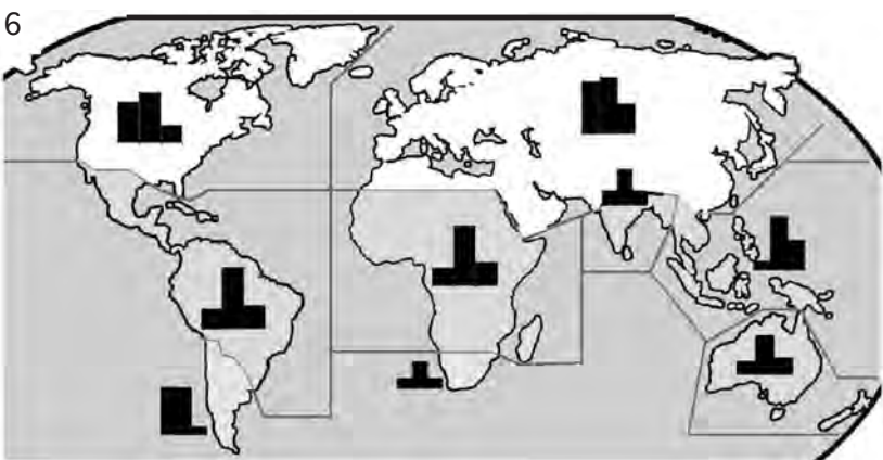
Figures 4–6. Geographic distribution patterns of quantitative vessel element features. – 4: Mean vessel diameter classes (includes diffuse porous, semi-ring porous, and ring porous woods). – 5: Vessels per sq. mm (only diffuse porous woods). – 6: Vessel element lengths.
